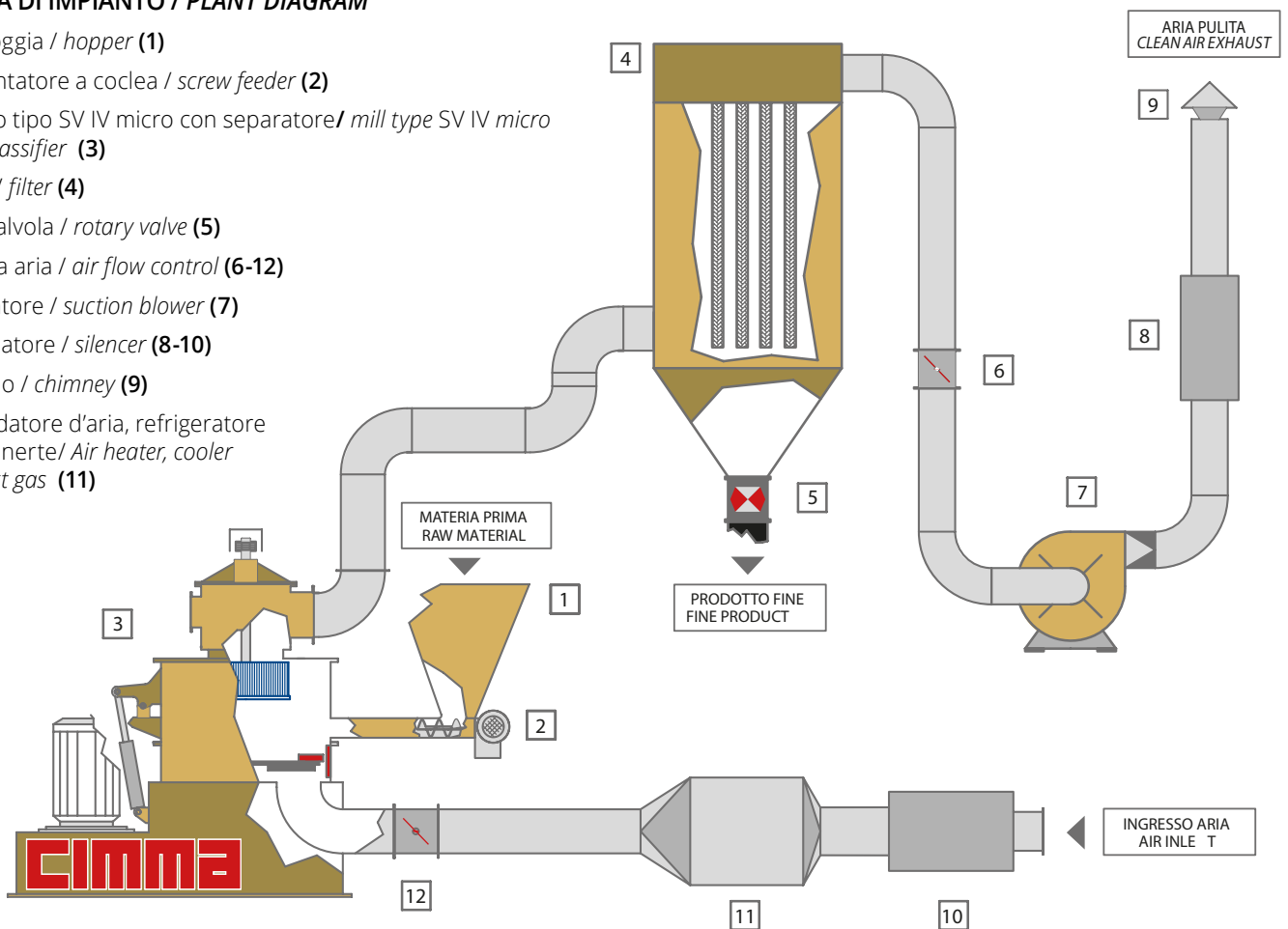
SV4 Micro graphite powder production plant
